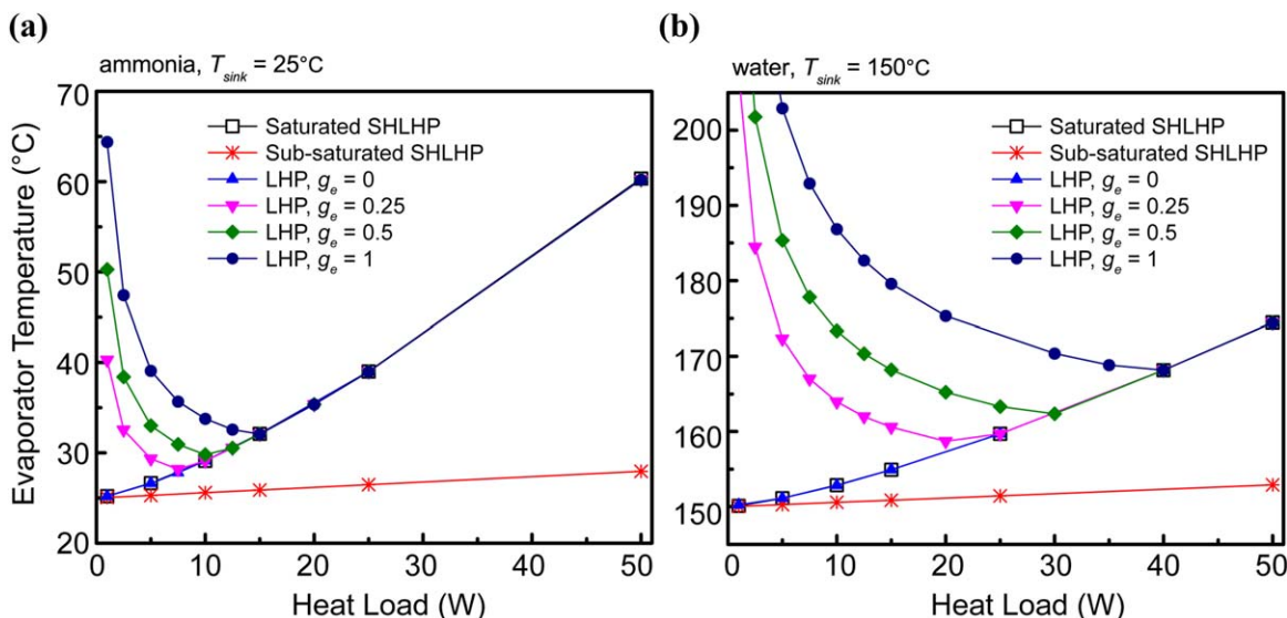
Figure 5. Effect of the adverse acceleration (ranging for 0–1 time gravity) on conventional LHP, saturated SHLHP and subsaturated SHLHP with (a) ammonia and (b) water as working fluid.
