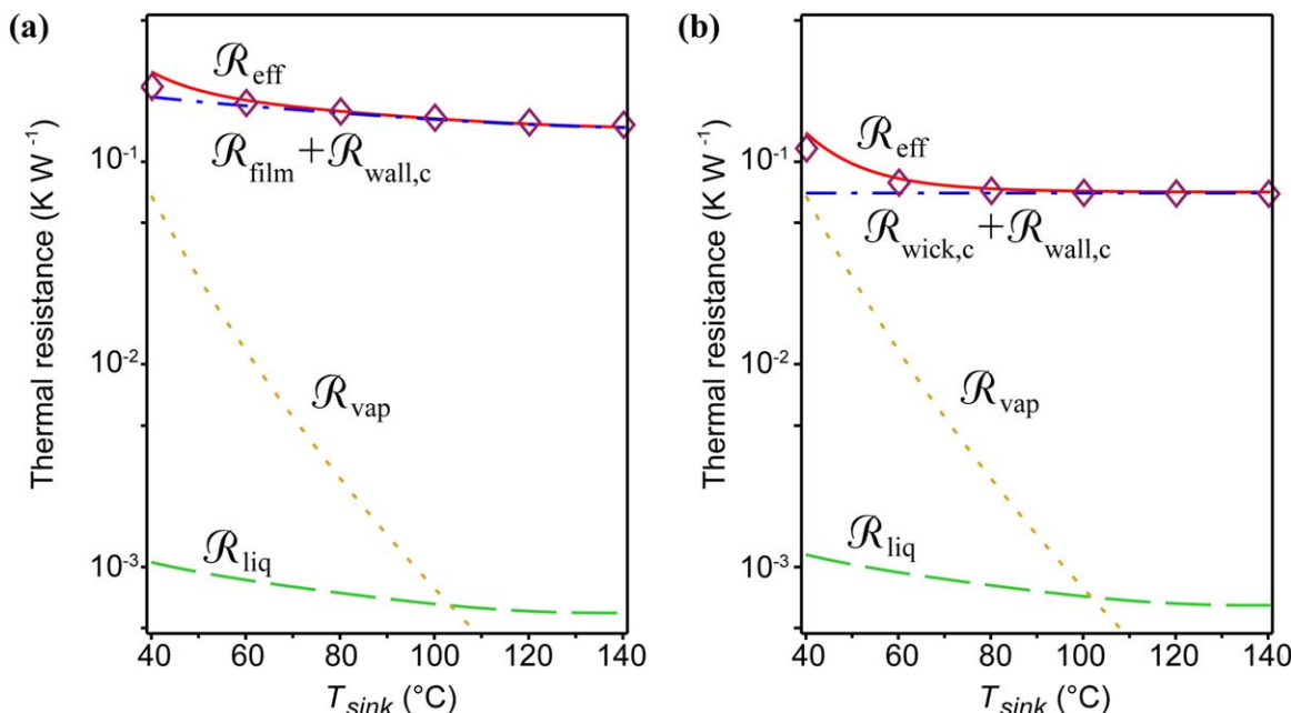
Figure 7. Predicted effective thermal resistances of (a) saturated SHLHP and (b) subsaturated SHLHP as a function of the sink temperature, T_{\text{sink}} .
