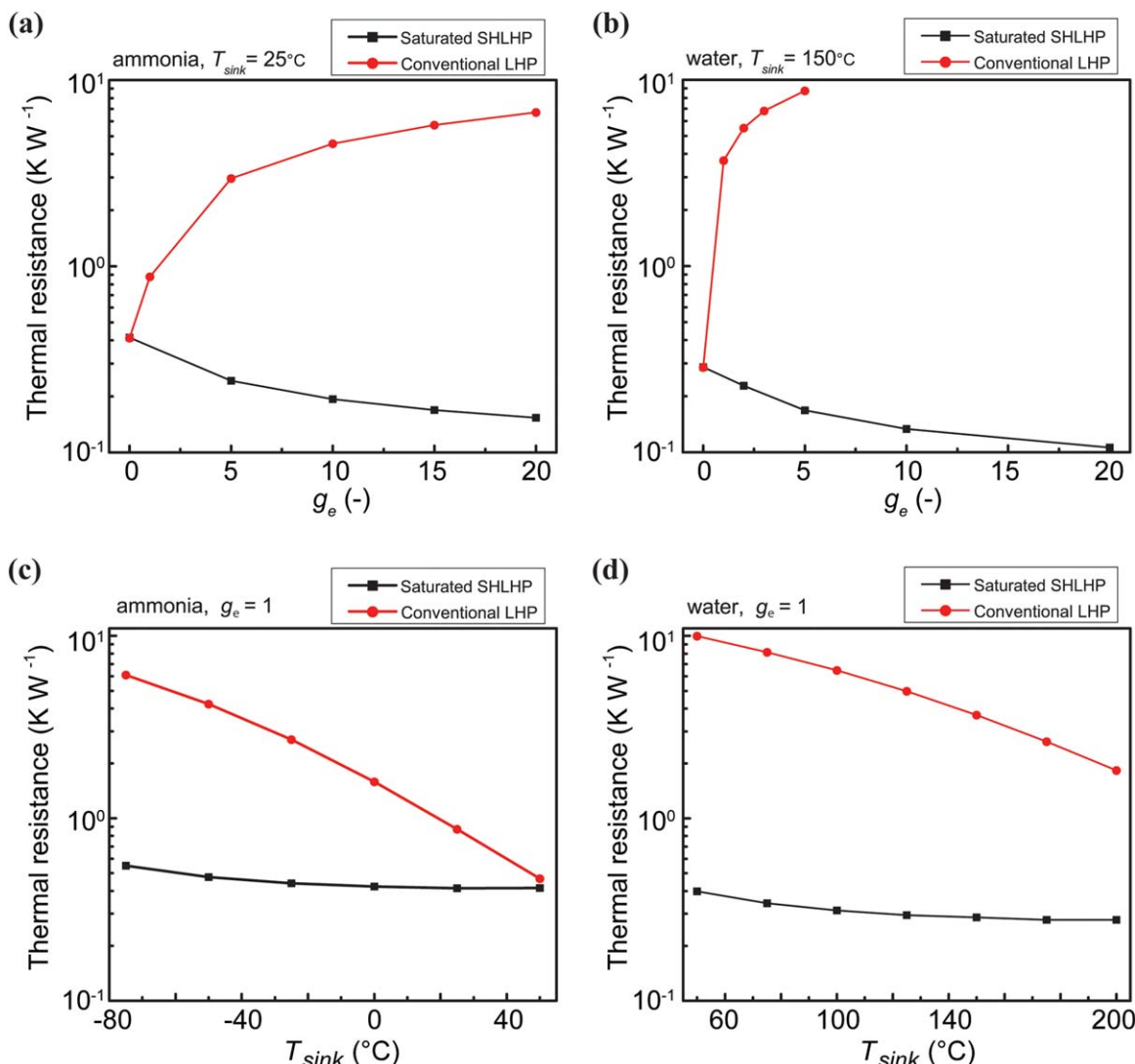
Figure 6. Comparison of the total effective thermal resistance for conventional LHP and saturated SHLHP varying acceleration (a–b) and sink temperature (c–d), with ammonia and water as the working fluid.
