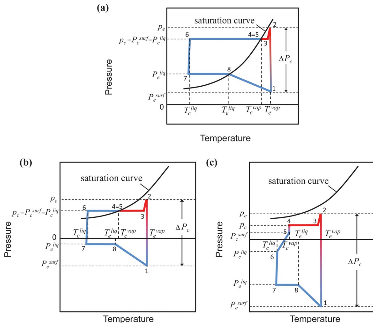
Figure 2. Schematic representations of working cycles on P - T diagram for (a) conventional LHPs, (b) saturated SHLHPs, and (c) subsaturated SHLHP.
