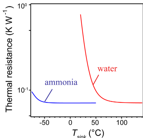
Figure 8. Total effective thermal resistances of subsaturated SHLHP (Eq. 14) with water (red curve) and ammonia (blue curve) as working fluid.
