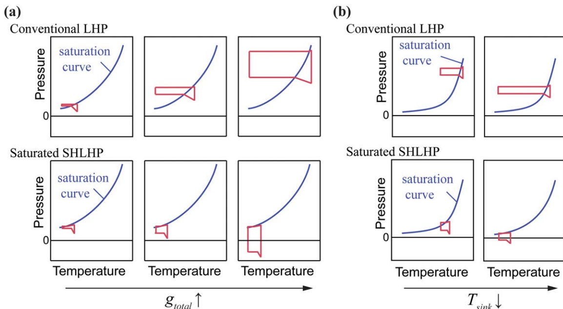
Figure 3. P - T diagrams for conventional LHP and SHLHP steady-state operation.
