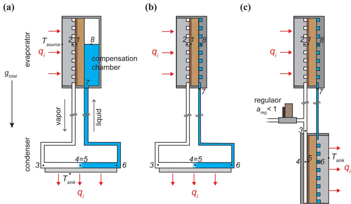
Figure 1. Schematic cross-sectional views of (a) a conventional LHP, (b) a saturated SHLHP, and (c) a subsaturated SHLHP.
