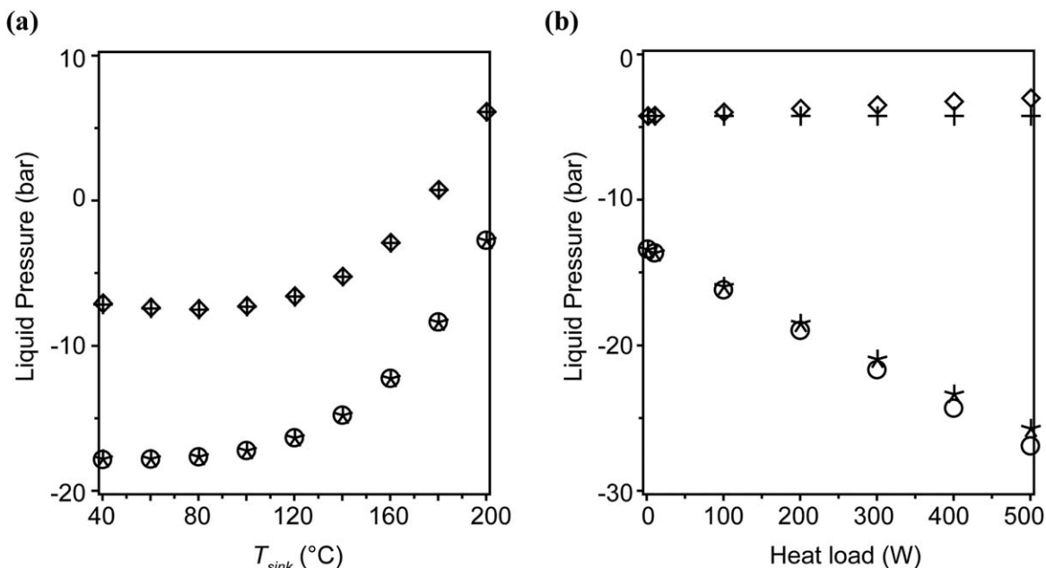
Figure 9. Liquid pressure profile in subsaturated SHLHP as a function of (a) sink temperature, T_{\text{sink}} , and (b) heat load.
