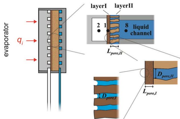
Figure 4. Schematic diagrams of the nanoporous membranes required in the evaporator of the saturated SHLHP and in both the evaporator and condenser of the subsaturated SHLHP.
